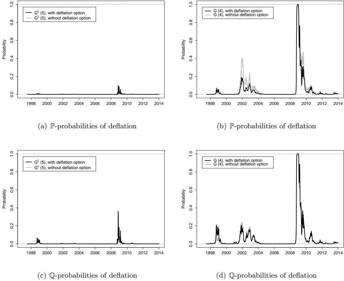
Figure 9: Estimated One-Year Deflation Probabilities
