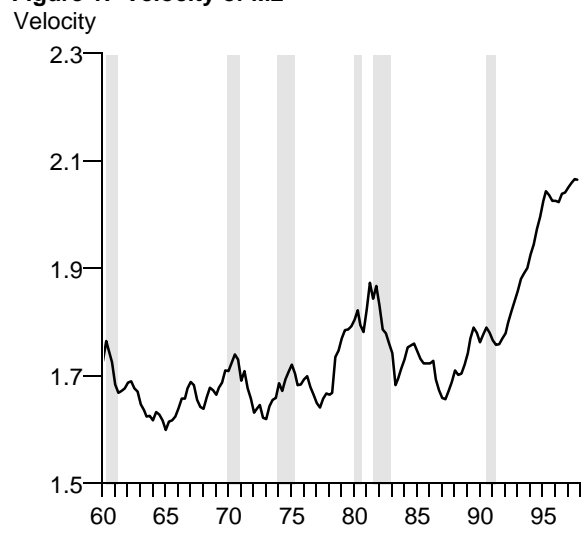
Figure 1: Velocity of M2
